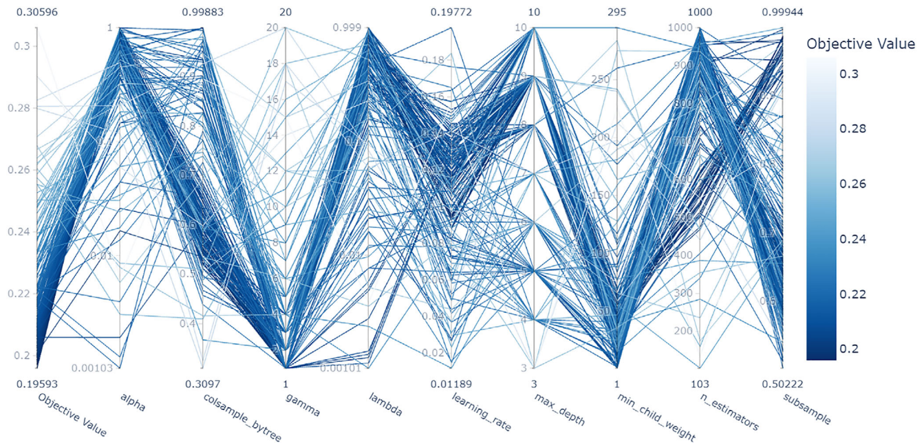
FIGURE 11 Parallel coordinate for the different hyperparameter values and the objective function values for XGBoost model
