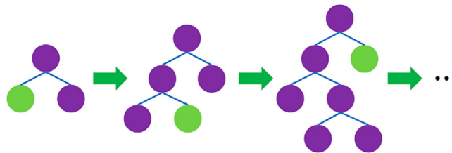
FIGURE 1 Leaf-wise tree growth strategy for LGBM algorithm
