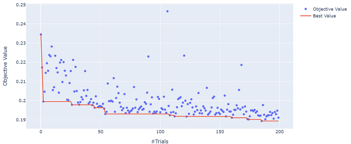
FIGURE 6 Optimization History for the LGBM Model over the 200 trials in minimizing the objective function
