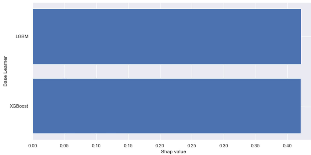
FIGURE 13 Contribution of each base learner to the overall output of the hybrid model in house price prediction
