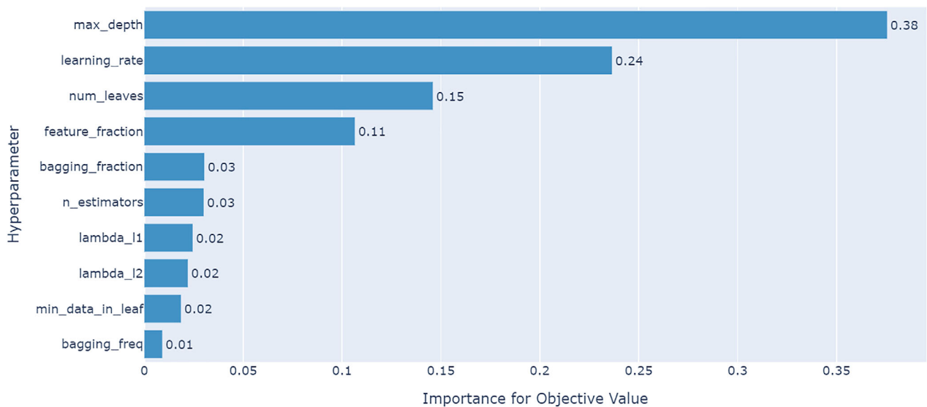
FIGURE 8 Hyperparameter importance in minimizing error for LGBM model
