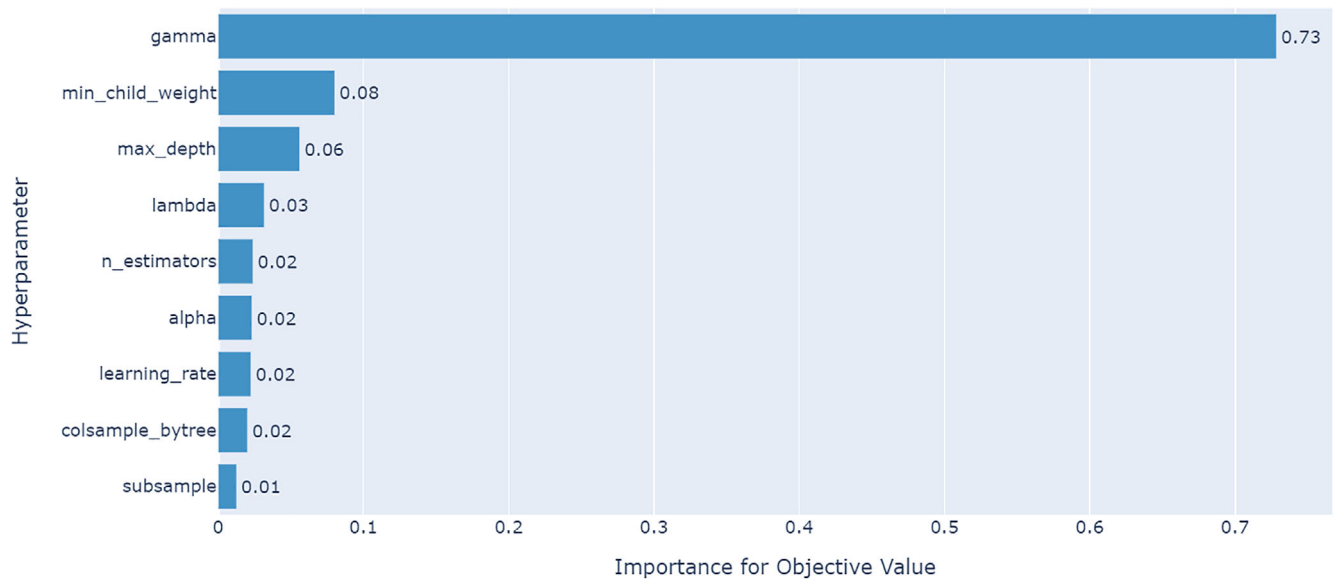
FIGURE 9 Hyperparameter importance in minimizing error for XGBoost model
