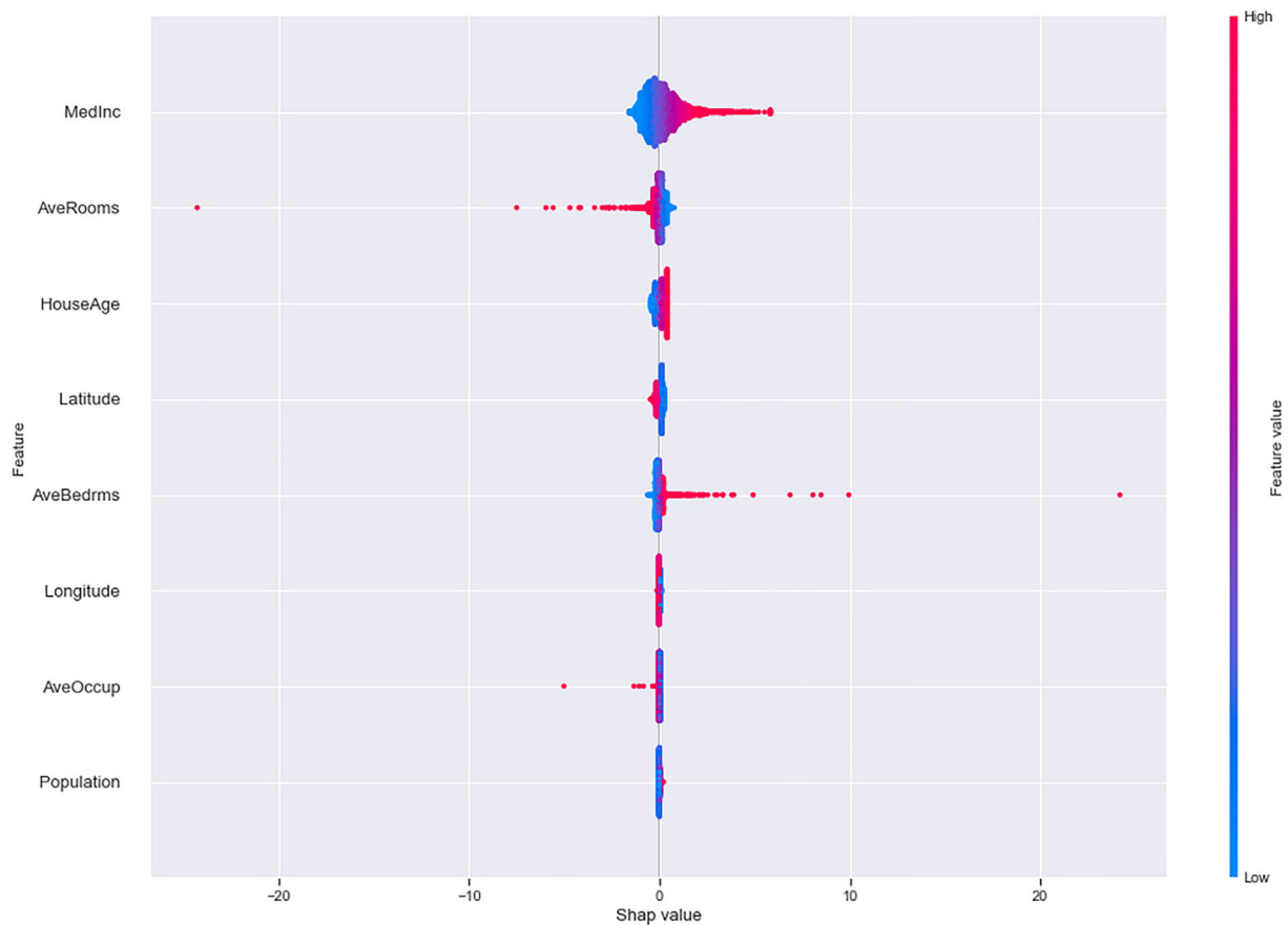
FIGURE 12 Hybrid Model Feature Importance Summary. The distribution and influence of the features in predicting house prices
