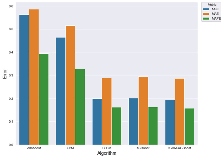
FIGURE 16 Performance evaluation of the proposed hybrid model. The hybrid LGBM and XGBoost model compared to Adaboost, GBM, LGBM, and XGBoost models
