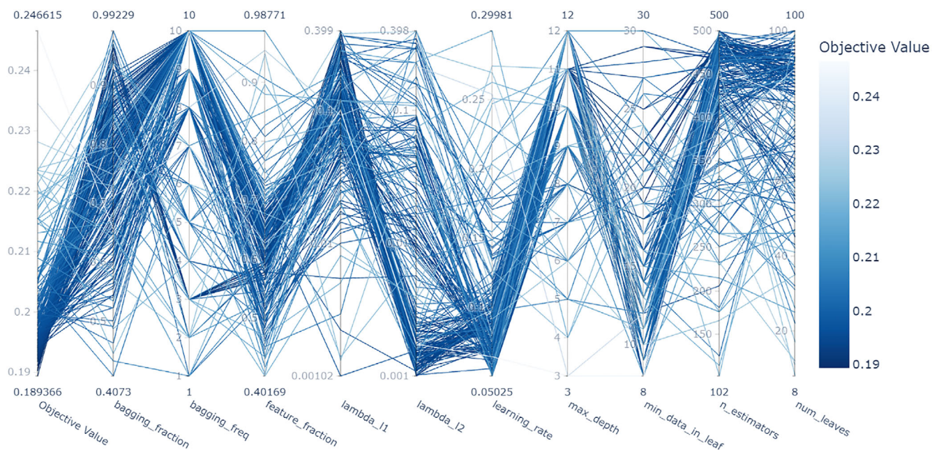
FIGURE 10 Parallel coordinate for the different hyperparameter values and the objective function values for LGBM model
