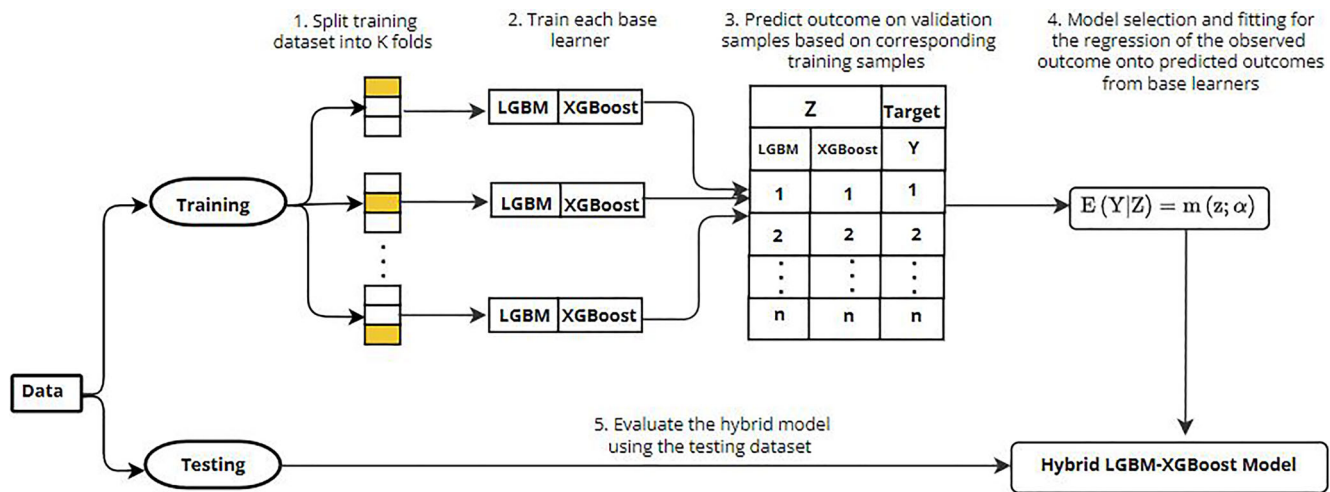
FIGURE 3 Flowchart which shows the implementation process of the proposed hybrid LGBM and XGBoost model
