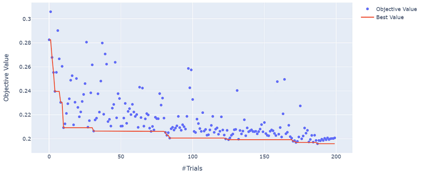
FIGURE 7 Optimization History for the XGboost Model over the 200 trials in minimizing the objective function
