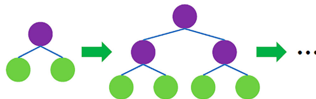
FIGURE 2 Level-wise tree growth strategy for XGBoost algorithm
