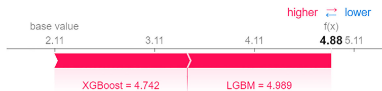
FIGURE 15 Hybrid model individual prediction explanation. The contribution of each base learner to the individual prediction
